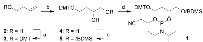
Scheme 1. Synthesis of phosphoramidite 1 for incorporation of \Delta . Reagents and conditions: a) DMT-Cl, pyridine, room temperature, 6 h, 99%; b) AD-mix- \beta , t BuOH, H 2 O, 0°C, 24 h, 73%; c) t BDMS-Cl, imidazole, CH 2 Cl 2 , room temperature, 16 h, 74%; d) (2-cyanoethyl) N,N -diisopropyl chlorophosphoramidite, Me 2 NEt, CH 2 Cl 2 , RT, 45 min, 75%.
