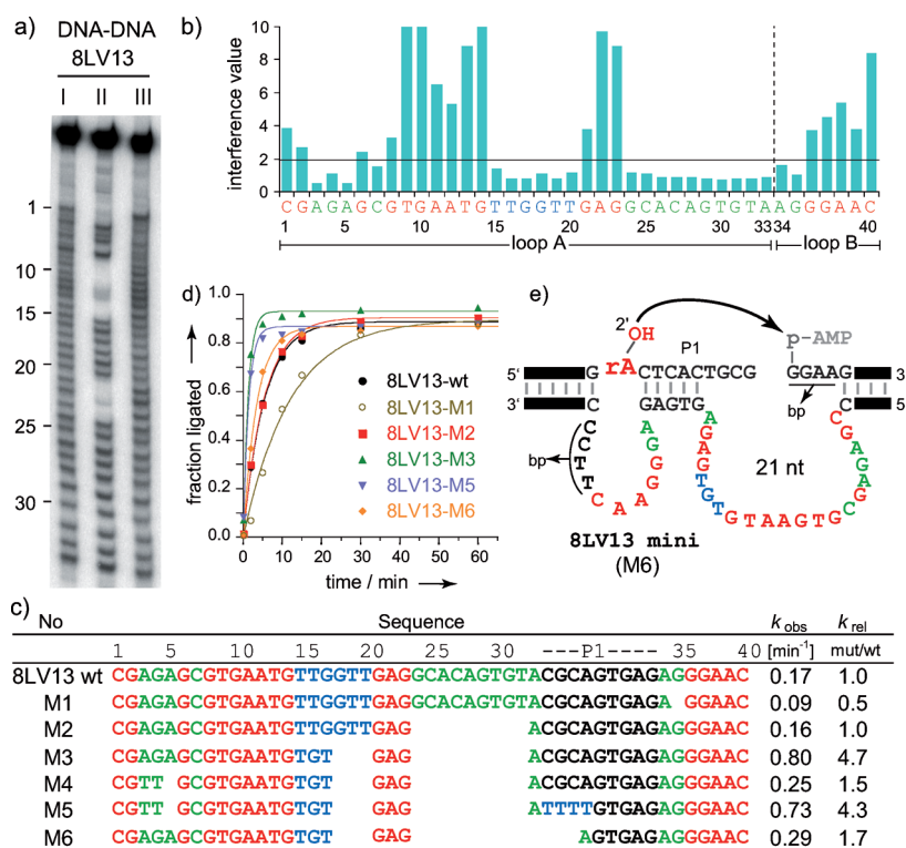
Figure 3. Combinatorial NDS mutagenesis for 8LV13-catalyzed DNA-DNA ligation. a) Hydrolysis gel for 33 nt-loop A (full gel in Supporting Information) Hydrolysis samples: I unselected library, II active fraction after ligation, 20 mM \text{Mn}^{2+} , pH 7.5, 37°C, 1.5 h. III unligated fraction. b) Interference values for each nucleotide; green: nucleotides with interference values less than 2, except nt 15–20 (see text for details), red: values over 2. c) Selection of mutants and their k_{\text{obs}} values. d) Kinetic plots for selected 8LV13 mutants. e) Minimized 8LV13 DNA (M6). wt = wild type.
