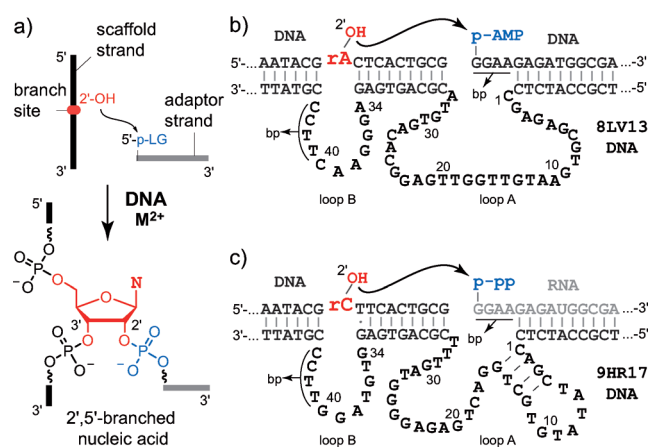
Figure 2. a) DNA-catalyzed synthesis of 2',5'-branched nucleic acids. b) 8LV13 deoxyribozyme for synthesis of 2',5'-branched DNA. [8] c) 9HR17 deoxyribozyme for connecting an RNA adaptor strand to a DNA scaffold strand. [12] The first four nucleotides of each adaptor strand form a base-paired (bp) region with the marked nucleotides of loop B to generate a three-helix junction structure. LG = leaving group.
